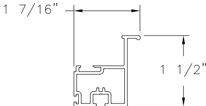
LIFT RAIL (BP4006) EXTRUDED RIGID PVC
