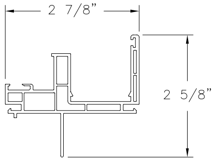
SILL (BP4002) EXTRUDED RIGID PVC
