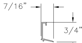
GLAZING BEAD (DT1720-R) EXTRUDED RIGID PVC
